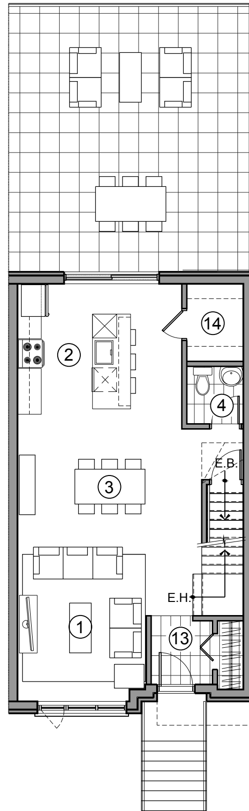
REZ-DE-CHAUSSÉE First Floor
